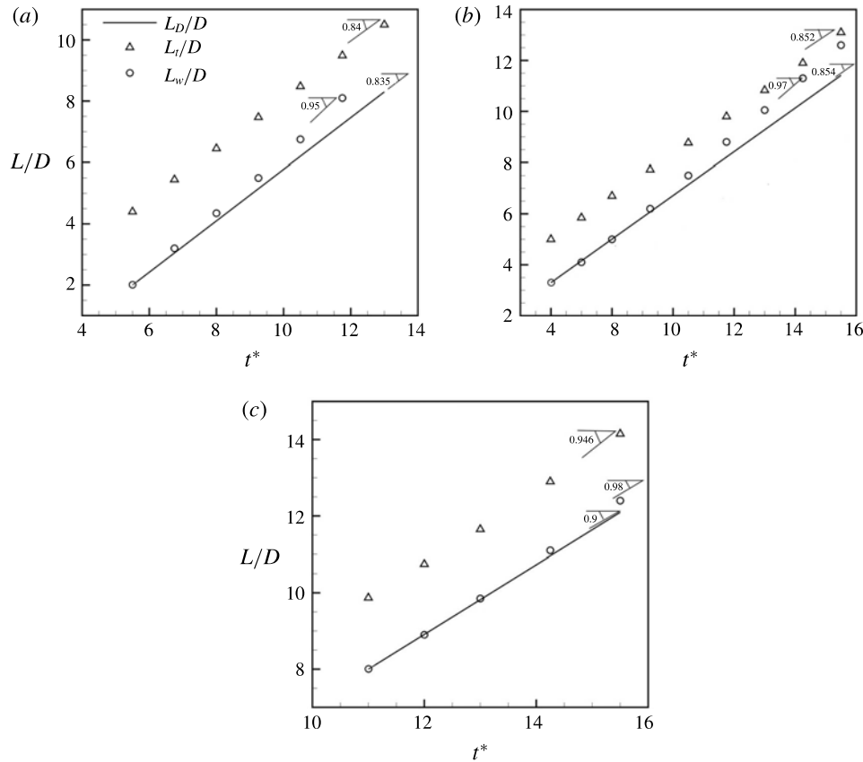
FIGURE 8. Temporal plot of L_t/D and L_w/D for case 1, \hat{U} = 0.1 (a); case 2, \hat{U} = 0.2 (b); and case 3, \hat{U} = 0.5 (c). The solid line indicates simple convection with Dimotakis velocity.
