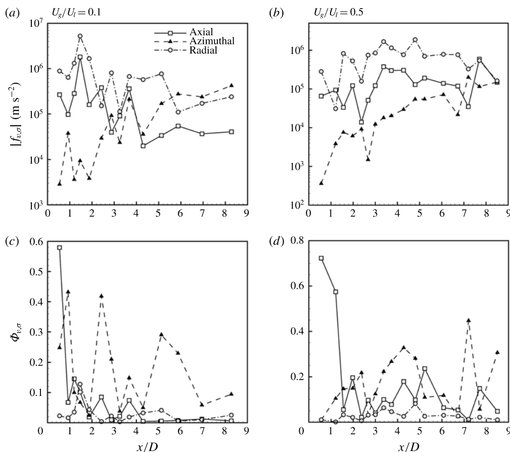
FIGURE 35. Comparison of viscous and surface tension forces, |f_{v,\sigma}| (a,b), and normalized viscous and surface tension forces, \Phi_{v,\sigma} (c,d), for case 1 (a,c) and case 3 (b,d), t^* = 11.5 .
