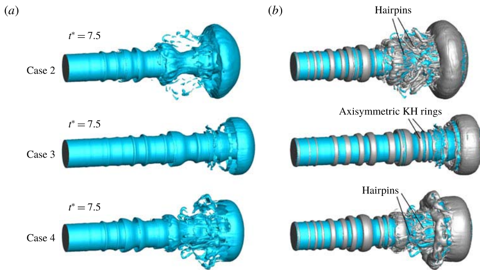
FIGURE 38. (Colour online) Liquid-jet surfaces (a), and the vortex structures (b) in case 2 (top), case 3 (centre) and case 4 (bottom); t^* = 7.5 .
