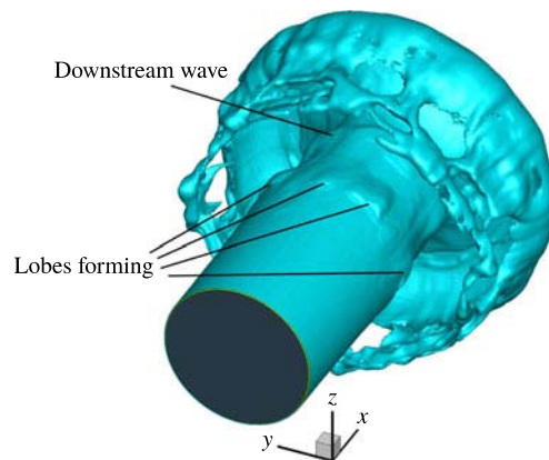
FIGURE 12. (Colour online) Liquid jet surface at t^* = 3.5 in case 2.
