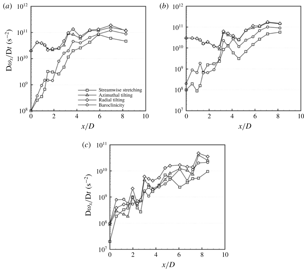
FIGURE 29. Contributions of streamwise vortex stretching (squares), azimuthal vortex tilting (triangles), radial vortex tilting (diamonds), and baroclinicity (circles) to the generation of \omega_x at the liquid surface for case 1 (a) case 2 (b) and case 3 (c); t^* = 11.5 .
