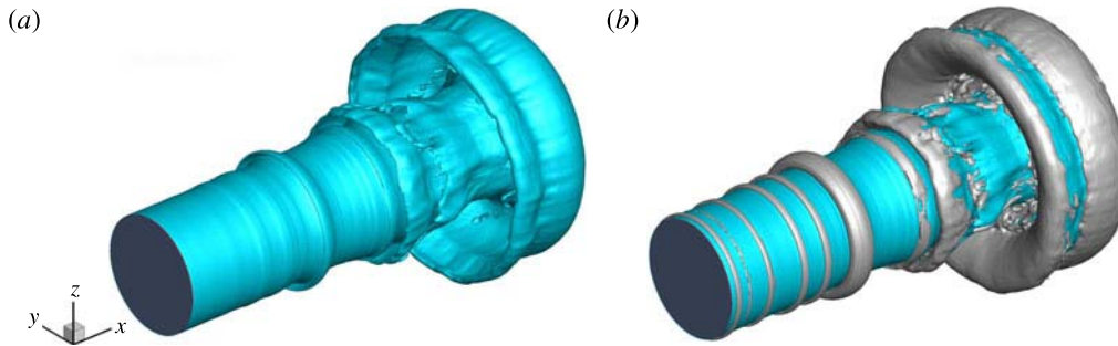
FIGURE 13. (Colour online) Liquid-jet surface (a); and vortex structures indicated by \lambda_2 = -10^{11} \text{ s}^{-2} isosurface (b) at t^* = 4.5 in case 1.
