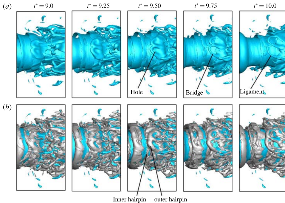
FIGURE 20. (Colour online) Step-by-step tracking of hole formation mechanism in case 1. Liquid surface on a thinning lobe subject to hole formation (a); vortex structures indicated by \lambda_2 = -10^{11} \text{ s}^{-2} isosurface on the same frame as 'a' (b). Time is indicated at the top of each column.
